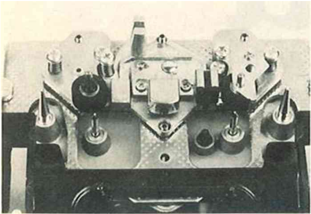
"DUAL CAPSTAN" s k Closed-loop-system.
