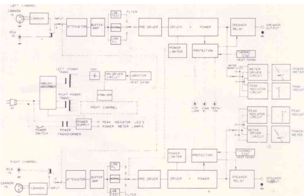
Linear complete-mirrored parallel push-pull circuitry
