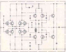
MC head amp circuit diagram
