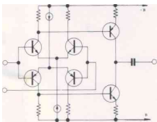
Linear complete-mirrored parallel push-pull circuitry
