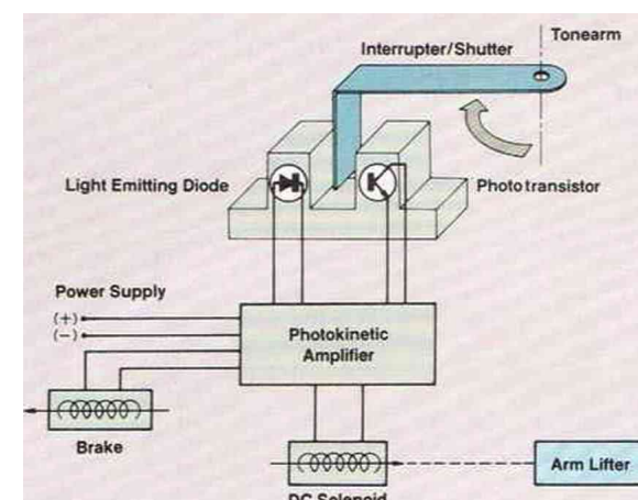
Block Diagram of JVC Photokinetic End-of-Play System
