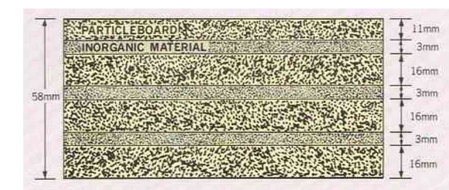
Cross Section of Multi-Layered Cabinet
