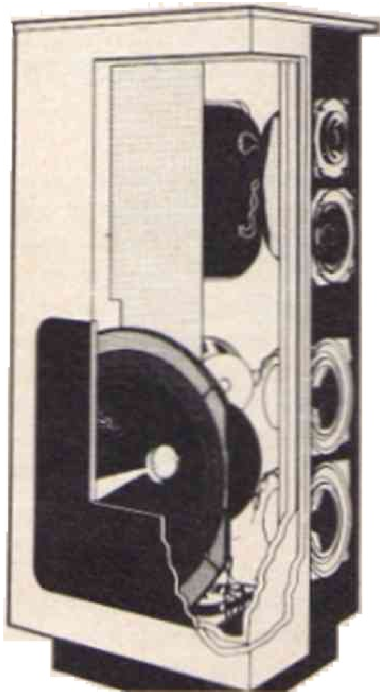
Goodmans Dimension 8 (cut-away)
